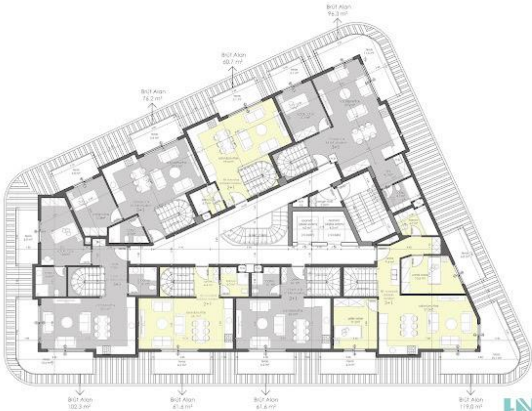
ÇATI KAT PLANI
